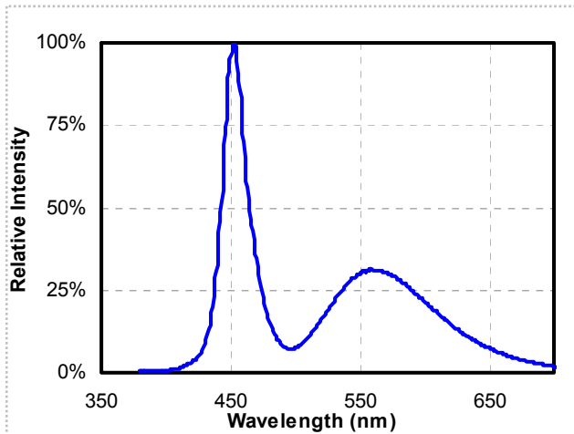
1. Spectrum Distribution ( T_A=25^\circ\text{C} , I_F=20\text{mA} )
